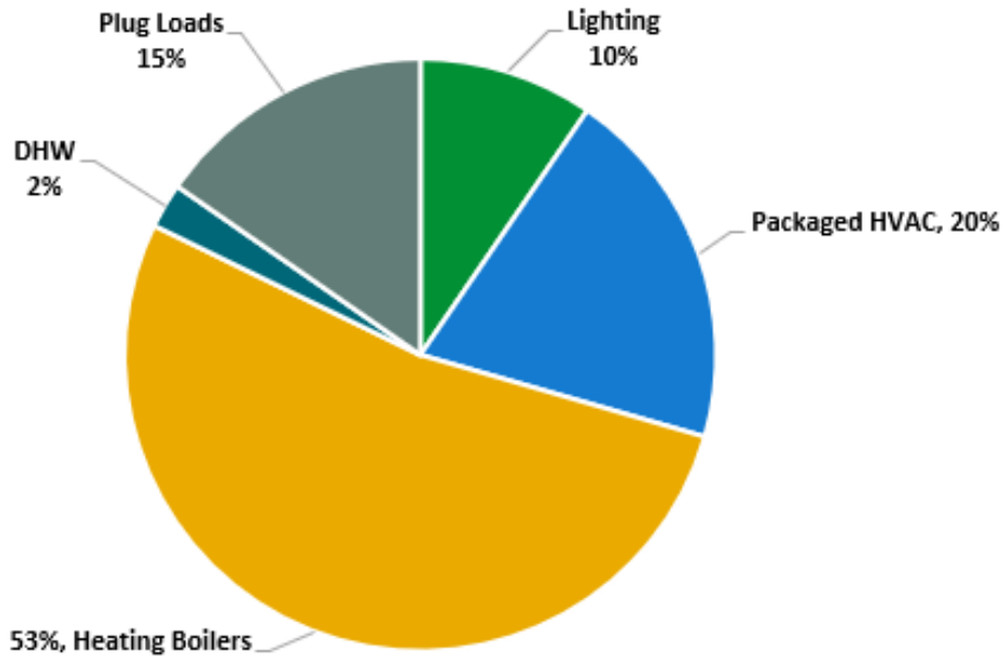
Energy Use by System
