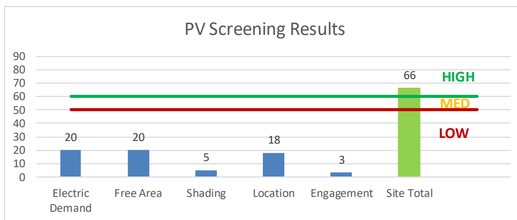
Figure 36 - Photovoltaic Screening
