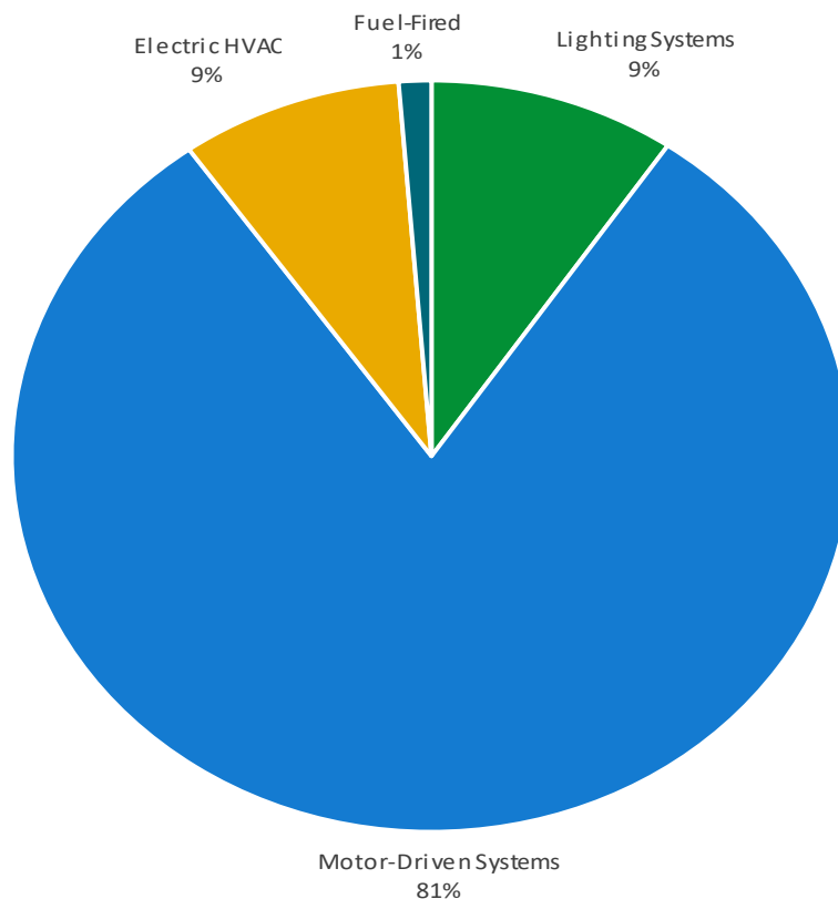
Figure 5 - Energy Balance
