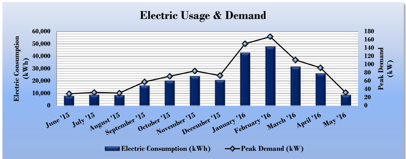
Figure 6 - Graph of 12 Months Electric Usage & Demand
