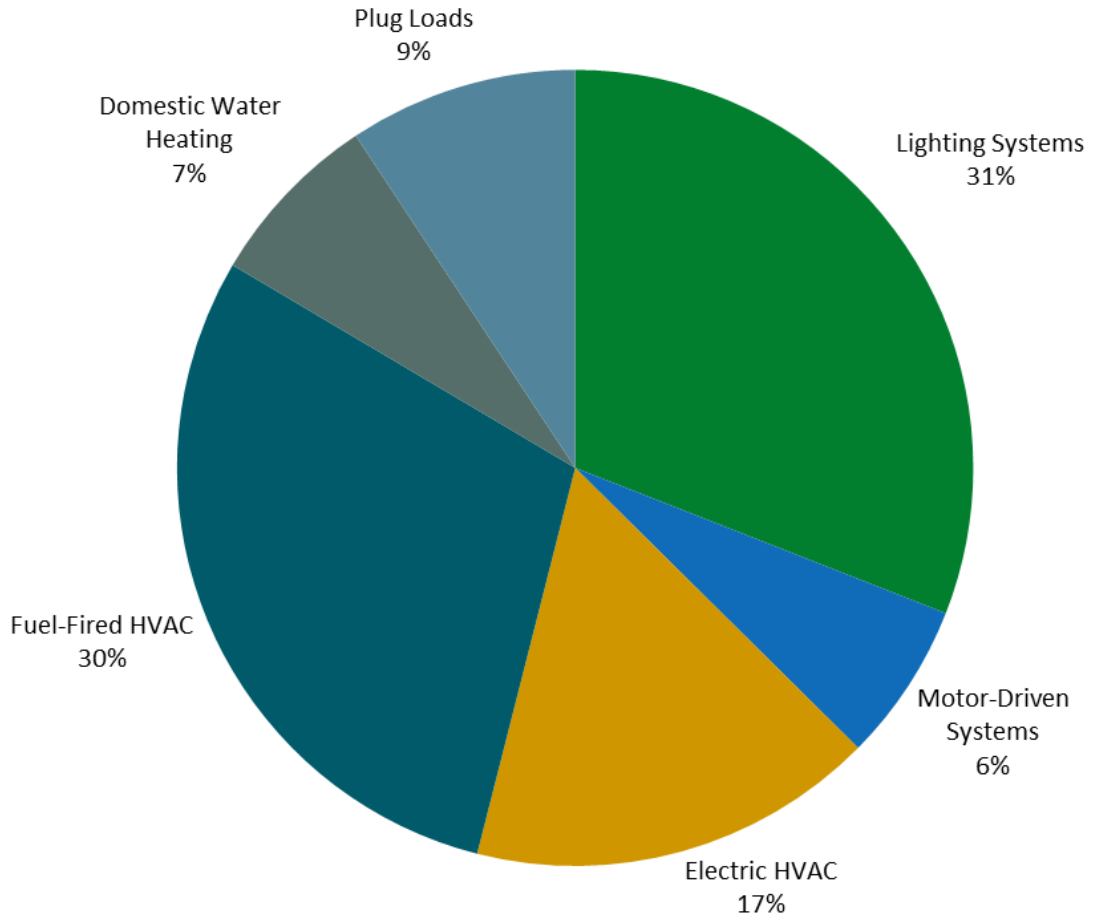
Figure 5 - Energy Balance
