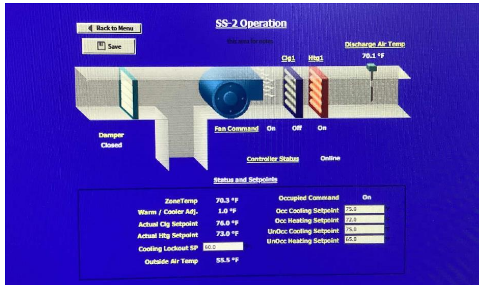
Air Handling Unit EMS Diagram View
