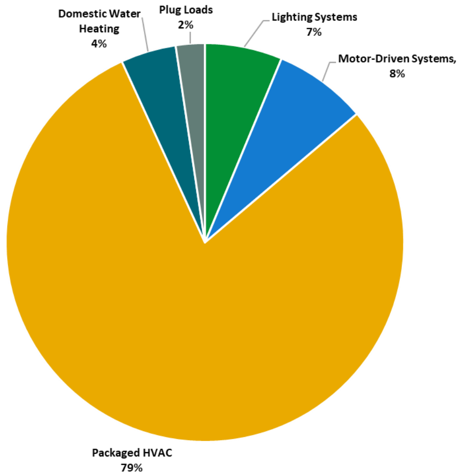
Figure 4 - Energy Balance
