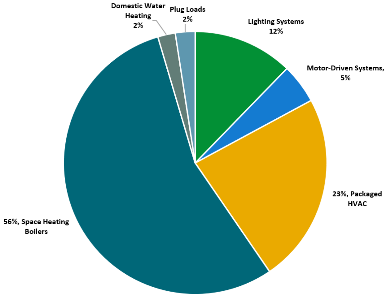
Figure 4 - Energy Balance
