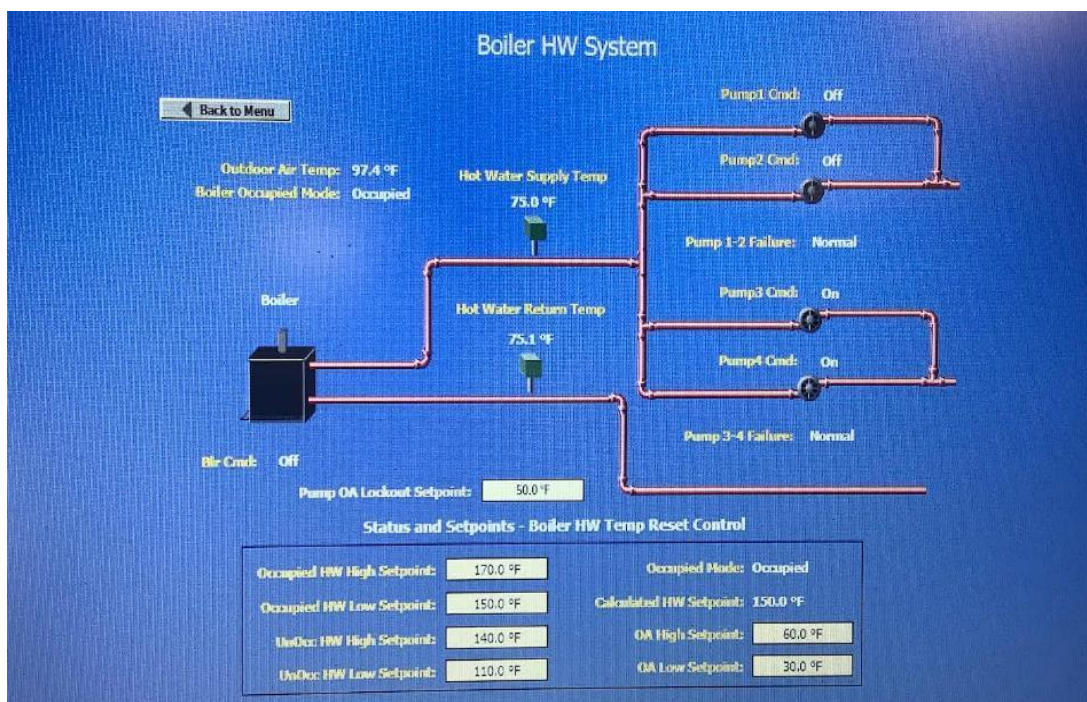
Heating Hot Water System EMS Diagram View
