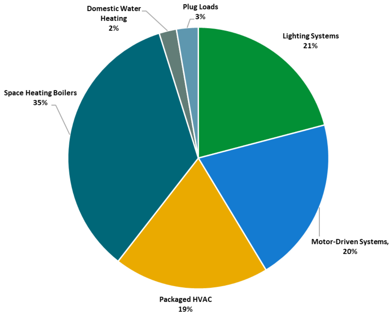
Figure 4 - Energy Balance
