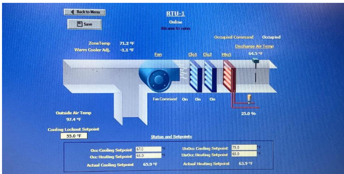
Package Rooftop Unit EMS Diagram View
