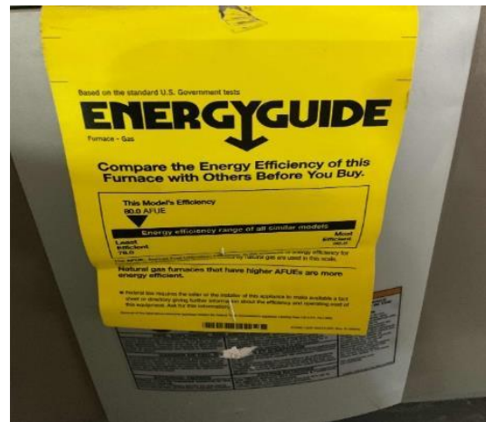
York Gas-Fired Furnaces
