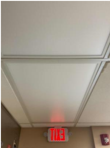
LED 2-foot x 4-foot Light Pane Fixture
