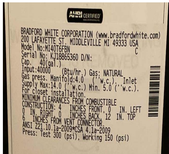
40-Gallon Gas Storage Tank Water Heater
