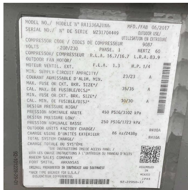
Rheem 3-ton Condenser Connected to AHU-2
