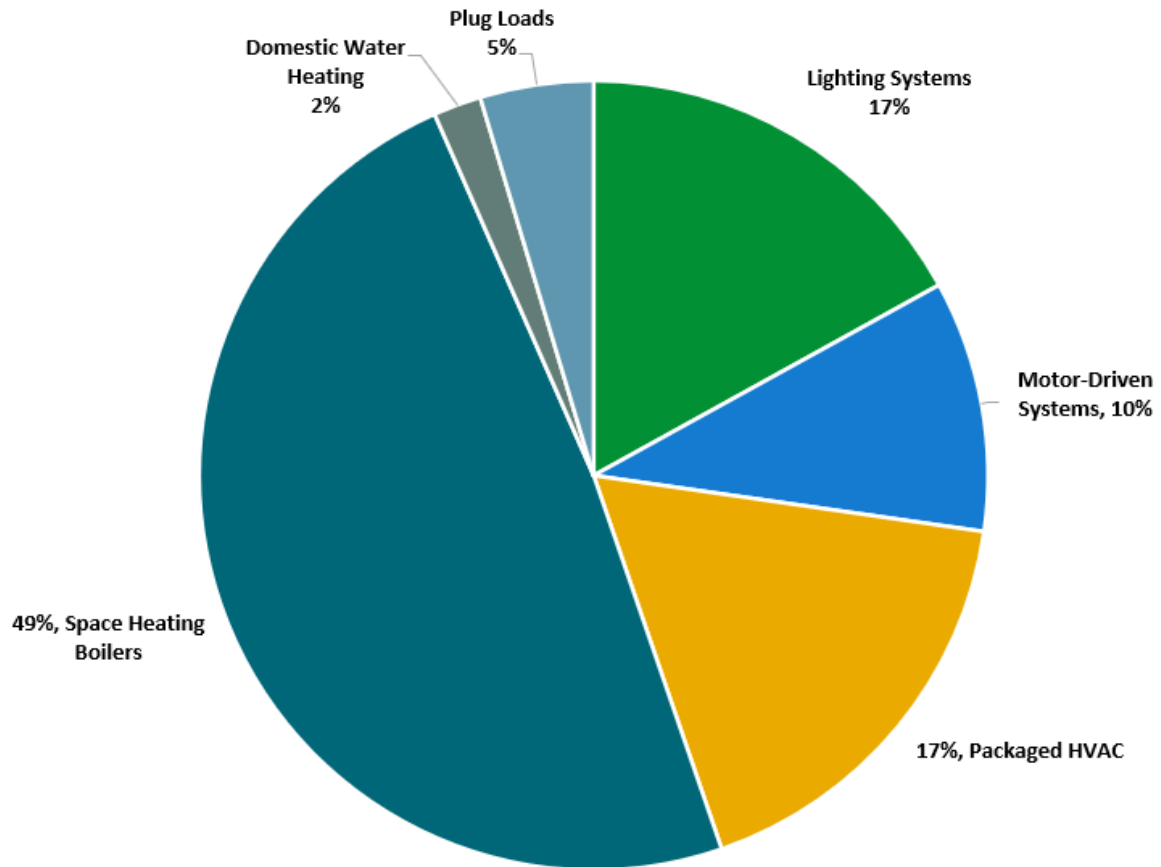
Figure 4 - Energy Balance
