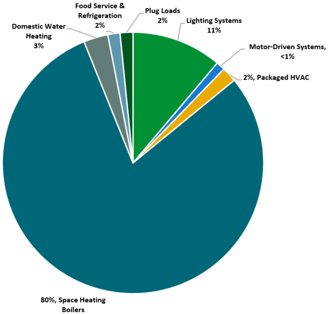
Figure 4 - Energy Balance
