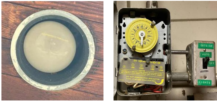
Exterior Recessed BR30 Incandescent Lamp & Timeclock
