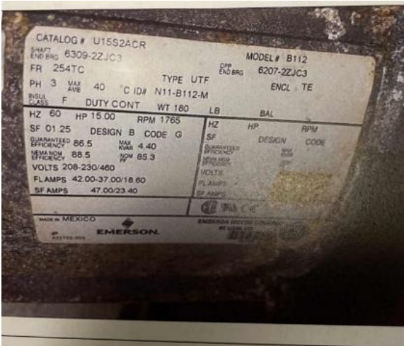
Original Sewer Ejector Name Plate
