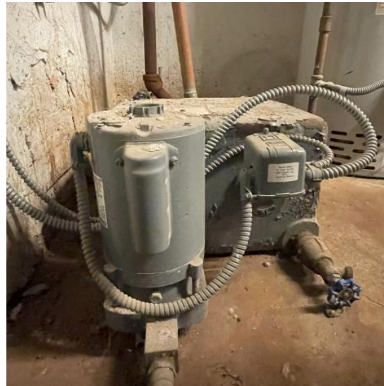
Condensate Pump
