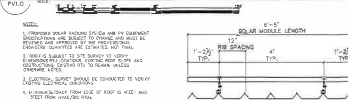
2 UNIRAC RACKING SYSTEM
