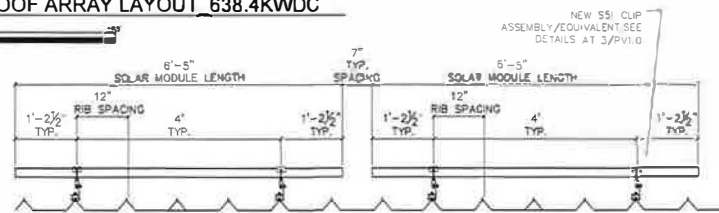
2 UNIRAC RACKING SYSTEM
