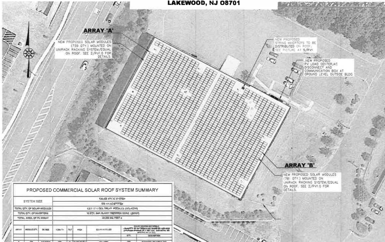
1 OVER-ALL SITE PLAN & PV ROOF ARRAY LAYOUT 638.4KWDC
