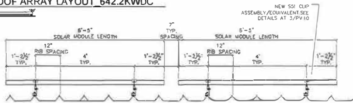
2 UNIRAC RACKING SYSTEM PV1.0 SCALE: 1/8\"/>
