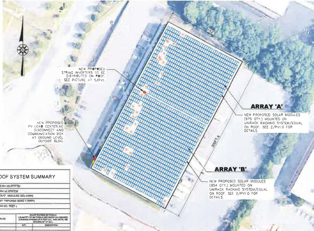
1 OVER-ALL SITE PLAN & PV ROOF ARRAY LAYOUT 642.2KWDC PV1.0 SCALE: 1" = 30' ±
