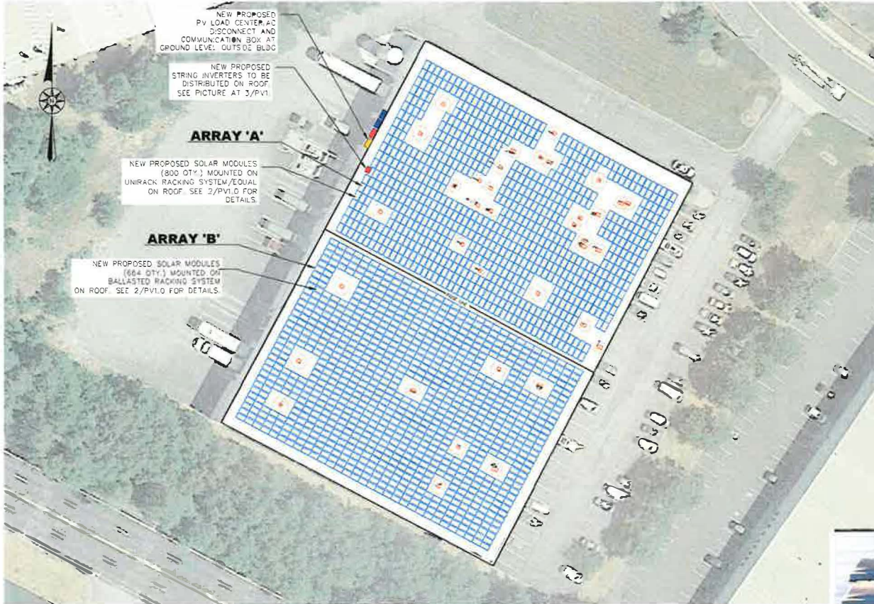
1 OVER-ALL SITE PLAN & PV ROOF ARRAY LAYOUT_714.2KWDC PV1.0 SCALE: 1/8"
