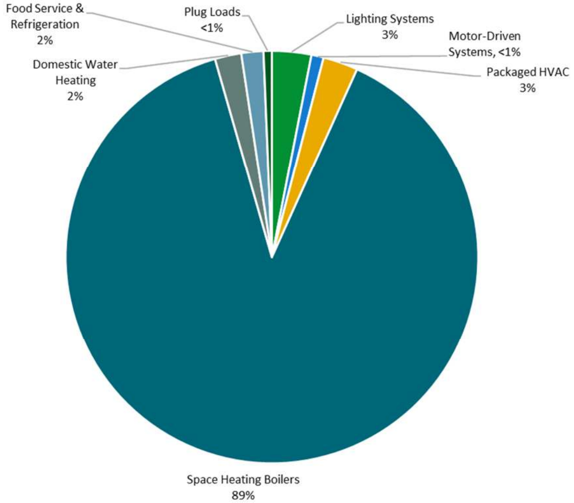
Figure 4 - Energy Balance
