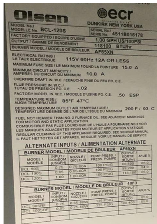
118 MBh Output Furnace Unit
